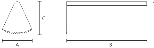
Blades for oscillating micro saw
